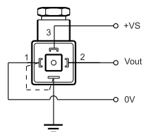
0-10V Output
